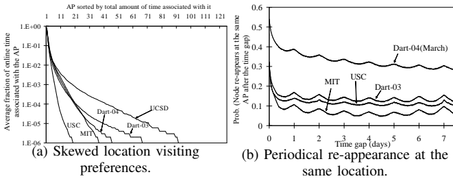
Fig. 1. Two important mobility features observed from WLAN traces.
