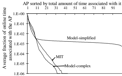
Fig. 7. Matching location visiting preferences of the synthetic traces to the WLAN trace.
